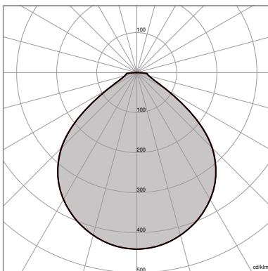
NEW WHITE 200
